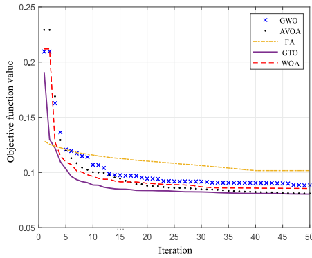
Figure 4. The convergence curve of the ITAE
